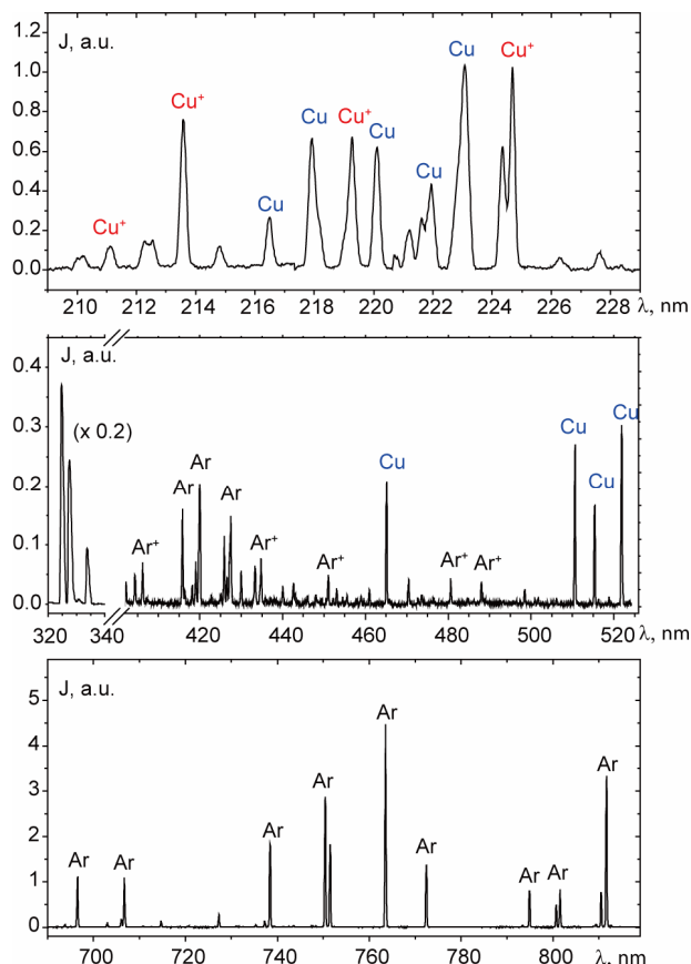
Figure 8. An optical emission spectrum from Ar/Cu plasma at wavelength between 210 and 830 nm. p = 5 \text{ mTorr} , I_{\text{el-mag}} = -0.4 \text{ A} , W = 3.36 \text{ kW} .
