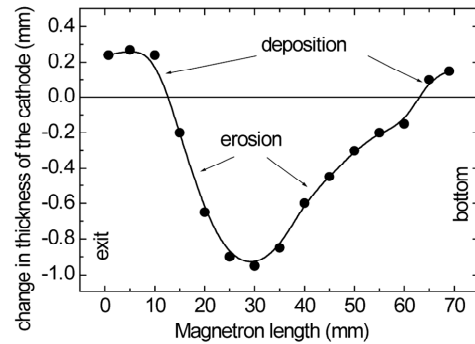
Figure 2. Structures of the target erosion.
