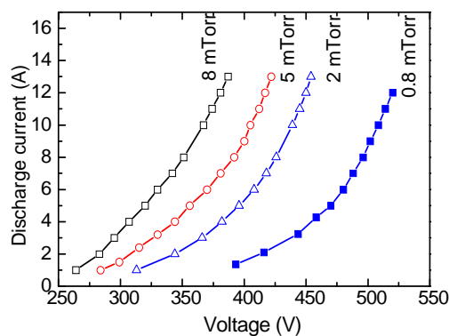
Figure 3. Current-voltage characteristics of the HCM for various pressures.
