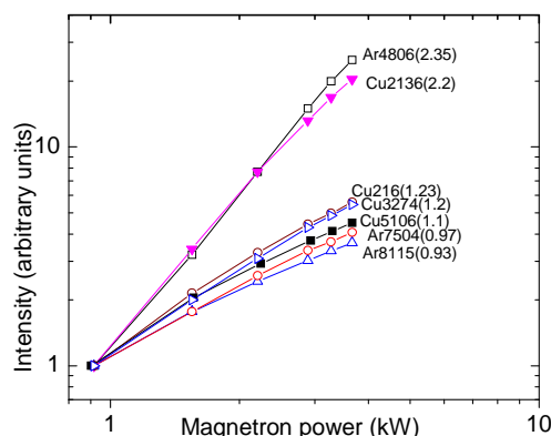
Figure 10. Normalized intensities of Ar and Cu spectral lines as function of a magnetron power, I_{\text{el}} = -0.5 A, 10 mTorr.
