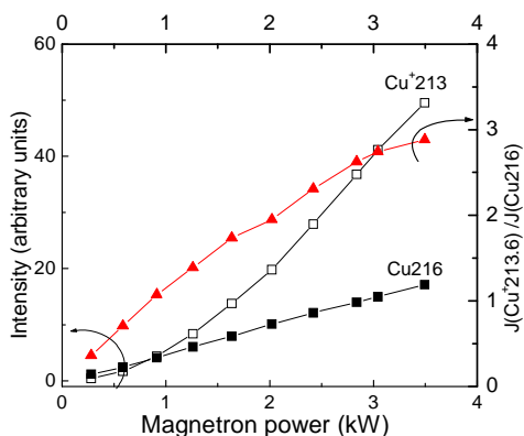
Figure 9. The optical emission intensities from Cu ion lines (213.6 nm) and Cu neutral (216.5 nm) at 10 mTorr vs discharge power.
