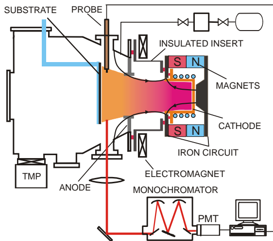
Figure 1. Schema of the experimental set-up.
