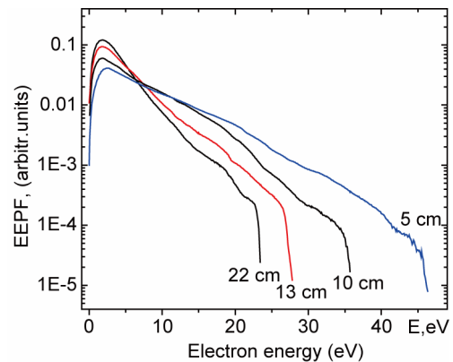
Figure 7. Normalized electron energy probability function on the discharge axis. p = 5 \text{ mTorr} , W = 1.3 \text{ kWatt} .
