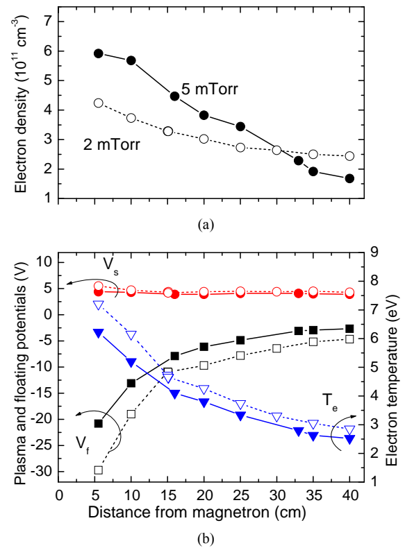
Figure 6. Axial distribution from the target exit of (a) Electron density N_e ; (b) Electron temperature T_e , plasma V_s and floating V_f potentials. I_{el-magn} = 0 \text{ A} . Solid lines: p = 5 \text{ mTorr} , I = 4 \text{ A} , U = 323 \text{ V} . Dot lines: p = 2 \text{ mTorr} , I = 4 \text{ A} , U = 370 \text{ V} .
