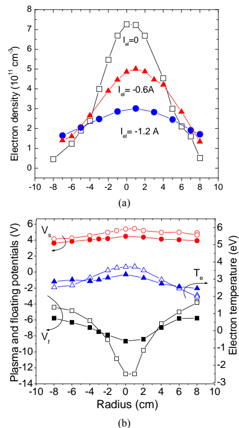
Figure 4. Radial profiles of: (a) The electron density N_e ; (b) Electron temperature T_e , floating V_f and plasma V_s potentials. 20 cm from the target. p = 10 mTorr, 50 sccm, W = 3 kWatt. Open symbols: I_{el} = 0 A, solid symbols: I_{el} = -0.6 A.
