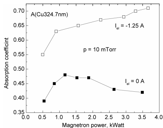
Figure 11. Absorption coefficient A of the Cu spectral line 324.7 nm as function of magnetron power.
