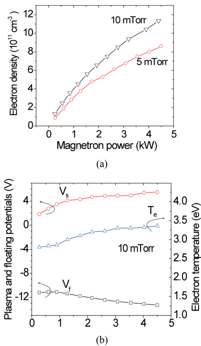
Figure 5. (a) Electron density; (b) Plasma potential V_s , floating potential V_f , and mean electron temperature T_e ; as function of the magnetron power. I_{el} = -0.6 \text{ A} . 20 cm from the target.
